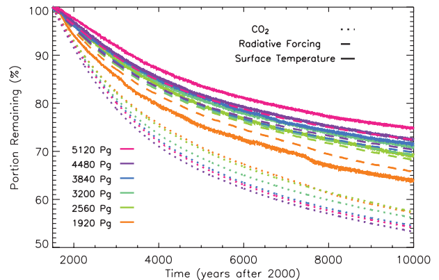
FIG. 12. Portion of anomalous \text{CO}_2 , radiative forcing, and surface temperature relative to 1500 yr after the start of the simulation. Although sometimes indistinct in the figure, the radiative forcing and temperature curves are similar: both show longer time scales (decline less steeply) than \text{CO}_2 and time scales become longer as emissions increase.
